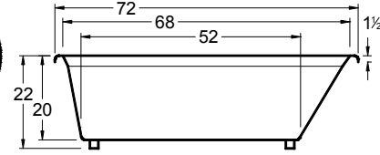
All bathtub dimensions are ± 1/2".
